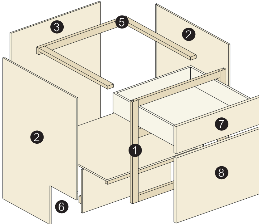
HANDICAP BASE CABINET CONSTRUCTION (32½" Height) STANDARD and DOMESTIC Option
